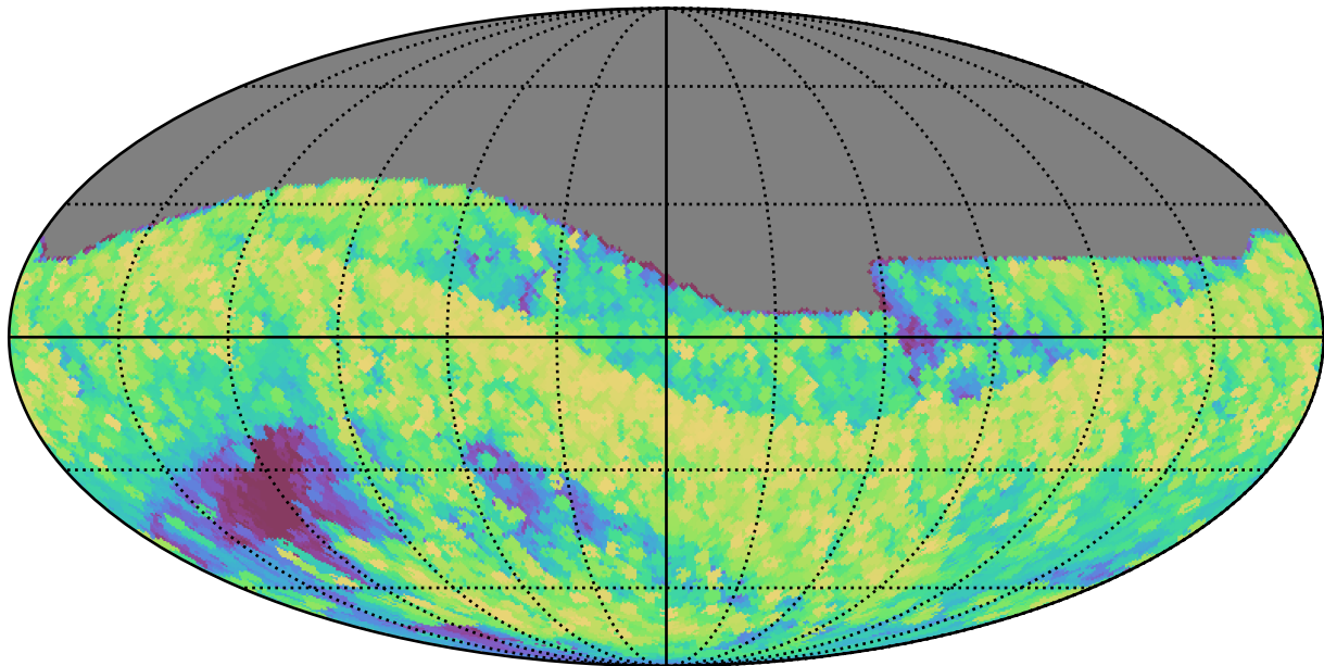
roll_pause_mjdp180_v3.4_10yrs All sky all bands: Max airmass
