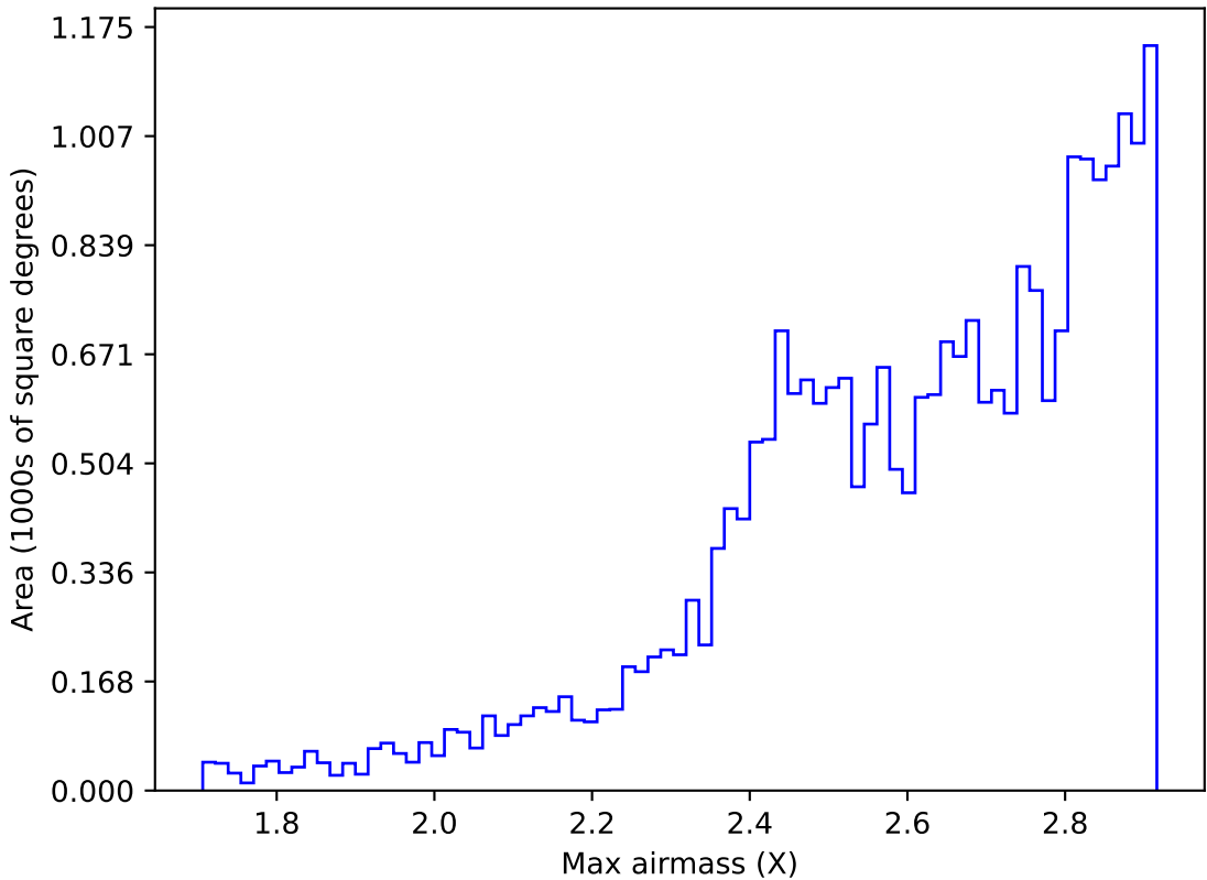
roll_pause_mjdp180_v3.4_10yrs All sky all bands: Max airmass
