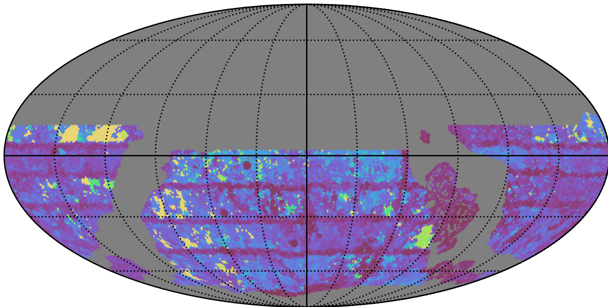
roll_pause_mjdp180_v3.4_10yrs WFD z band: Max Inter-Night Gap
