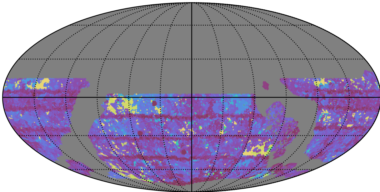
roll_pause_mjdp180_v3.4_10yrs WFD y band: Max Inter-Night Gap
