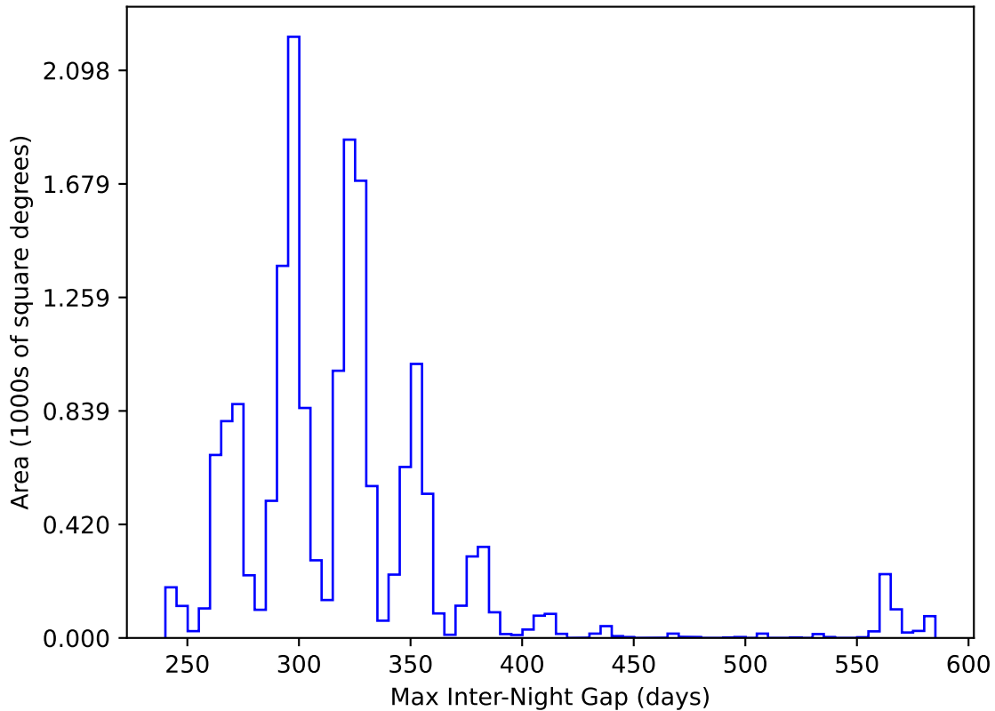
roll_pause_mjdp180_v3.4_10yrs WFD y band: Max Inter-Night Gap
