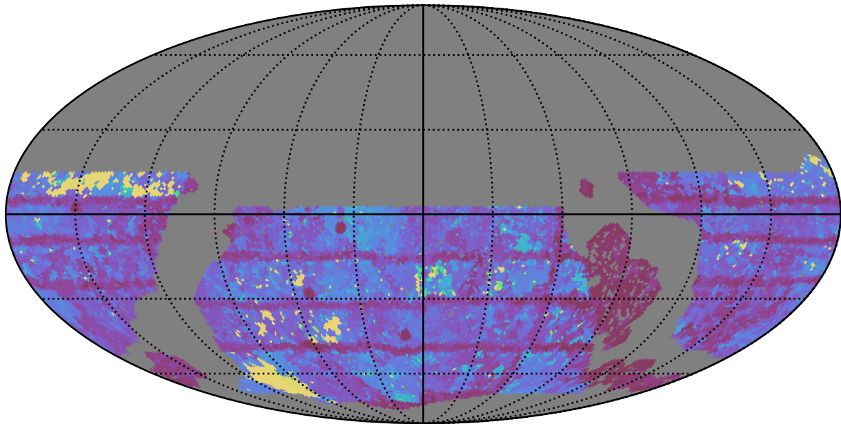
roll_pause_mjdp180_v3.4_10yrs WFD r band: Max Inter-Night Gap
