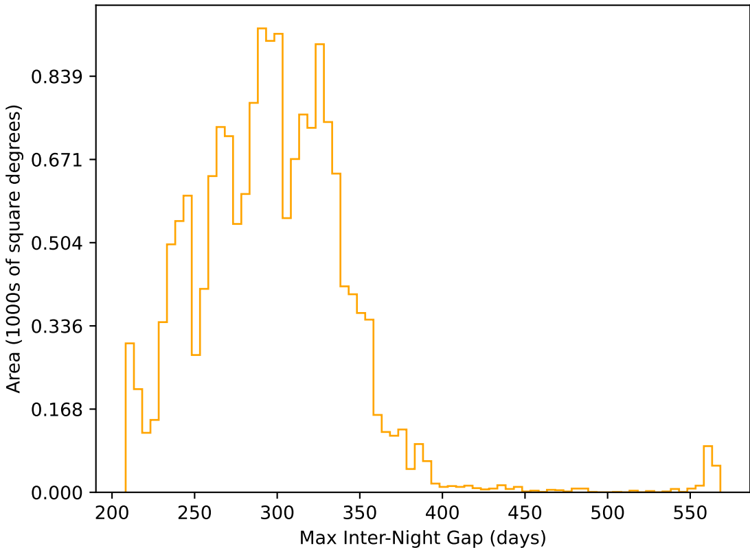
roll_pause_mjdp180_v3.4_10yrs WFD r band: Max Inter-Night Gap
