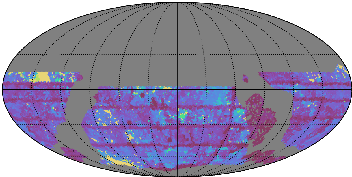
roll_pause_mjdp180_v3.4_10yrs WFD i band: Max Inter-Night Gap
