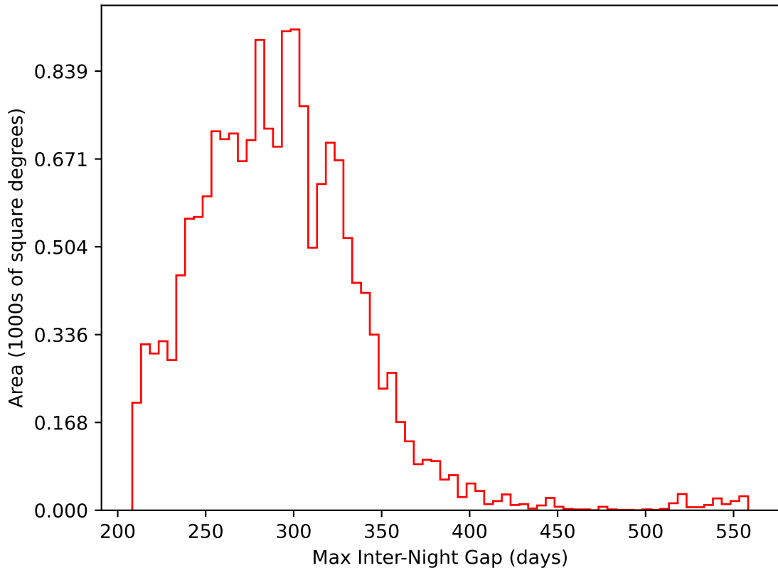
roll_pause_mjdp180_v3.4_10yrs WFD i band: Max Inter-Night Gap
