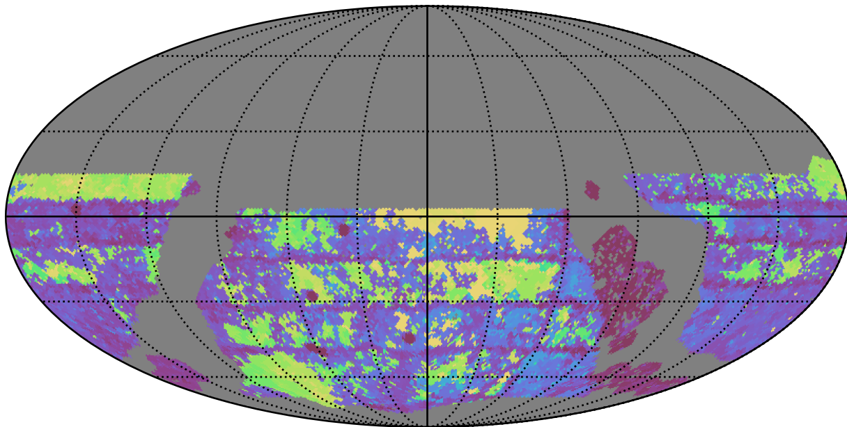
roll_pause_mjdp180_v3.4_10yrs WFD g band: Max Inter-Night Gap
