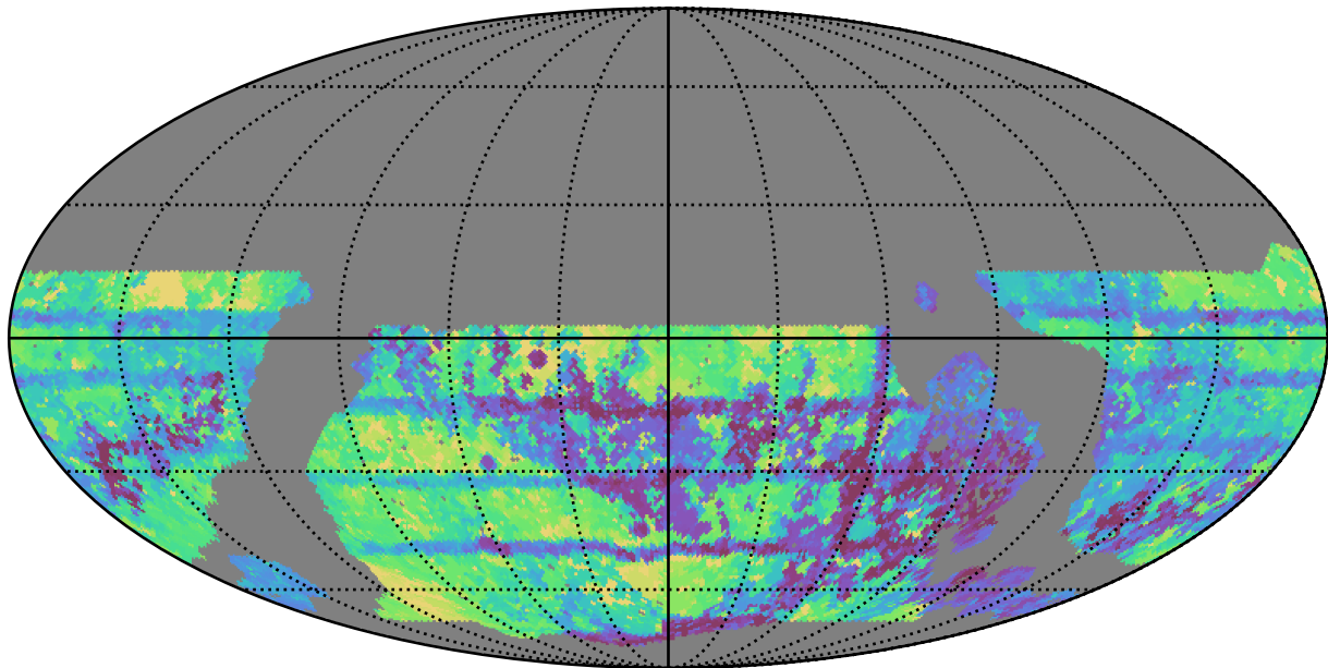
roll_pause_mjdp180_v3.4_10yrs WFD all bands: Max Inter-Night Gap
