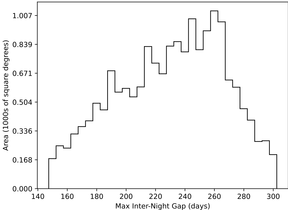
roll_pause_mjdp180_v3.4_10yrs WFD all bands: Max Inter-Night Gap
