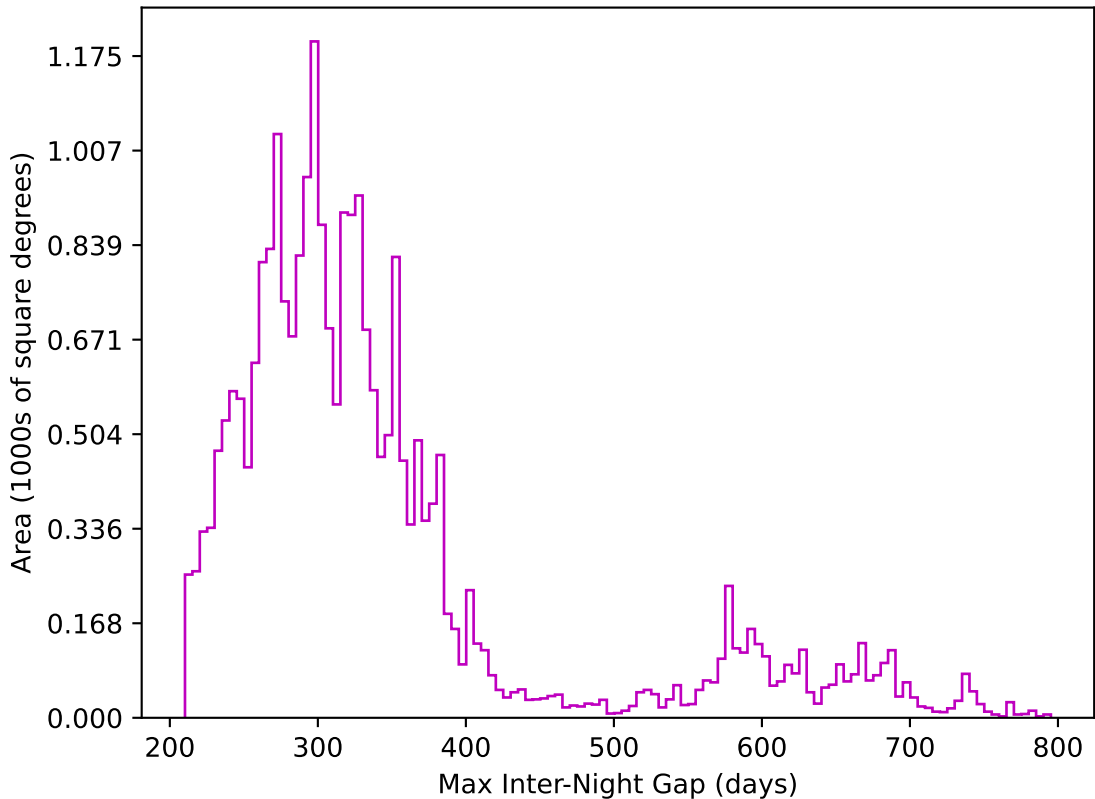
roll_pause_mjdp180_v3.4_10yrs All sky z band: Max Inter-Night Gap
