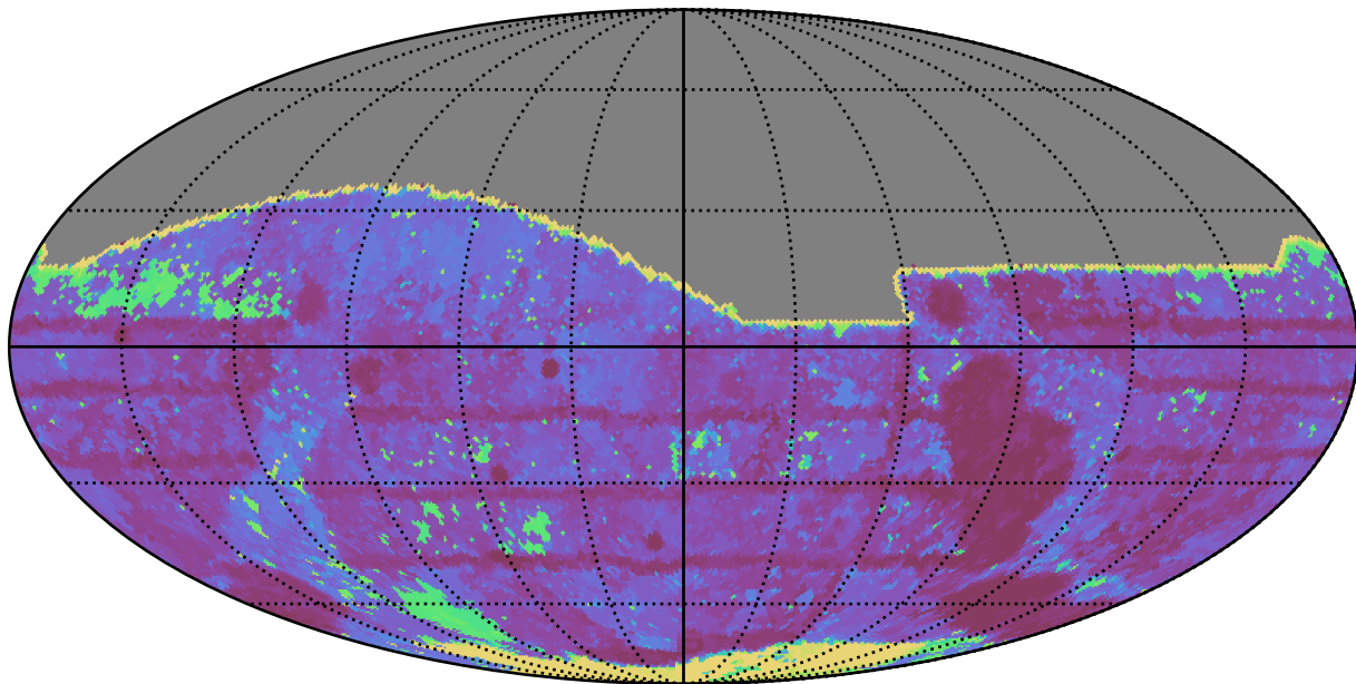
roll_pause_mjdp180_v3.4_10yrs All sky r band: Max Inter-Night Gap
