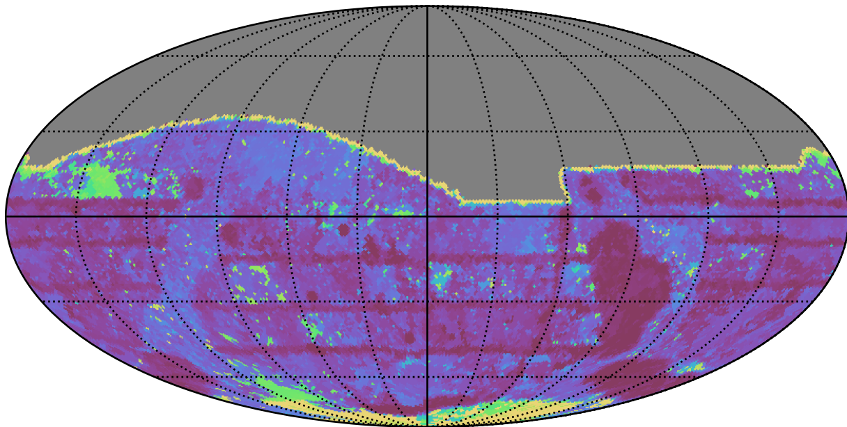
roll_pause_mjdp180_v3.4_10yrs All sky i band: Max Inter-Night Gap
