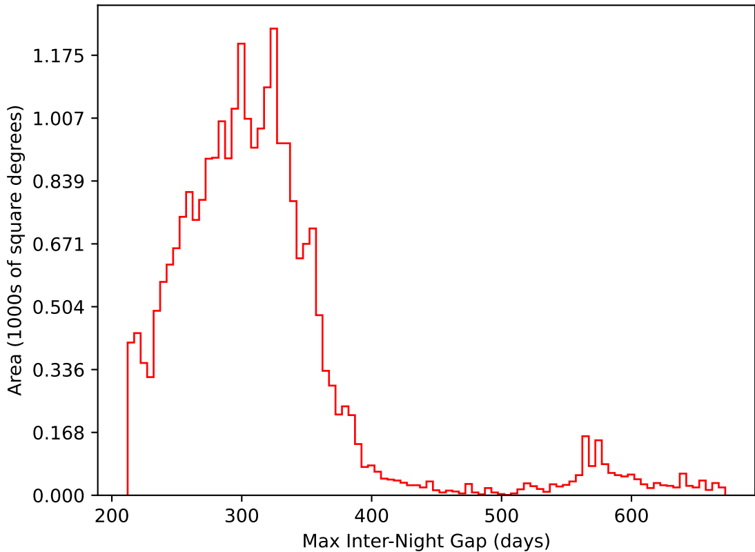
roll_pause_mjdp180_v3.4_10yrs All sky i band: Max Inter-Night Gap
