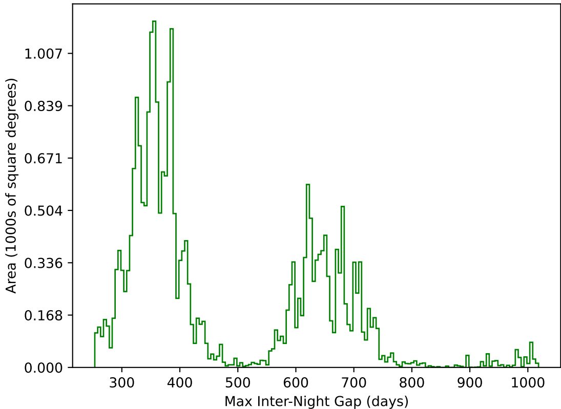
roll_pause_mjdp180_v3.4_10yrs All sky g band: Max Inter-Night Gap
