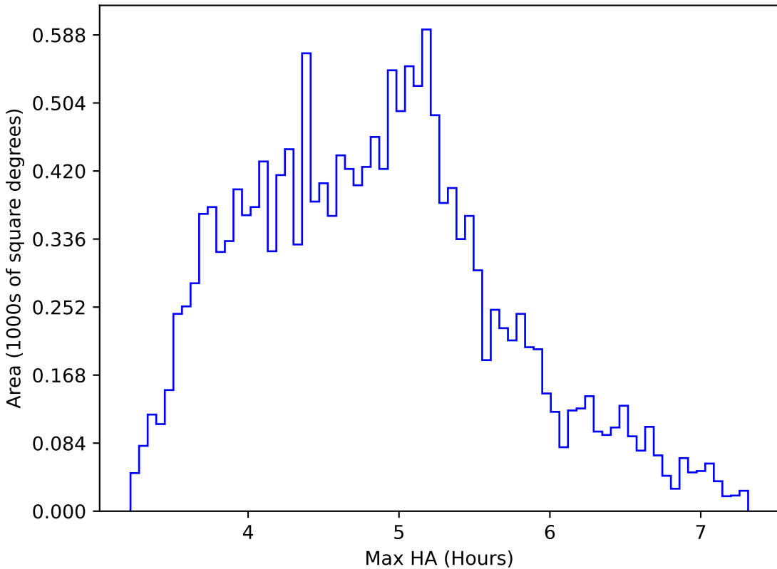
roll_pause_mjdp180_v3.4_10yrs WFD z band: Max HA
