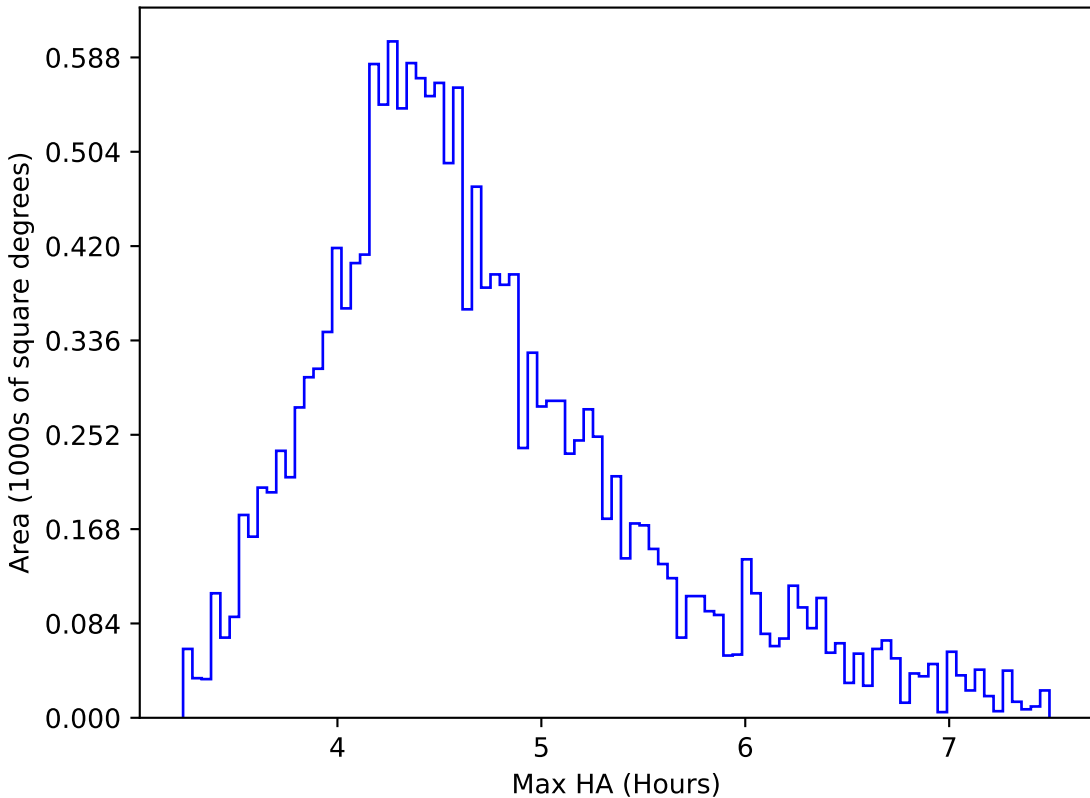
roll_pause_mjdp180_v3.4_10yrs WFD y band: Max HA
