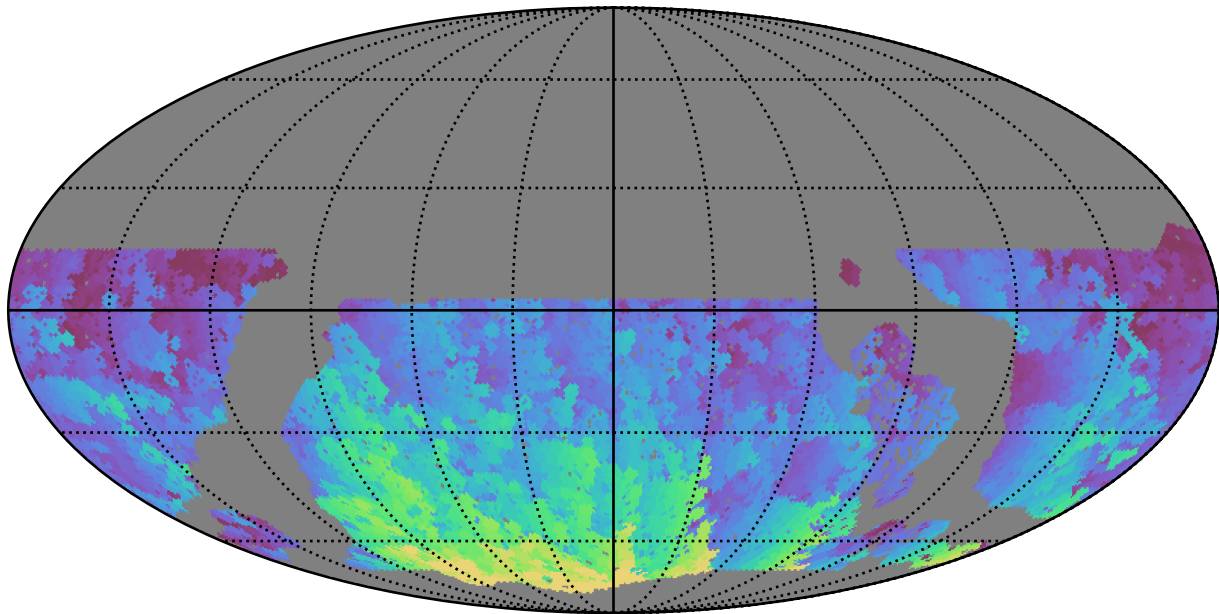
roll_pause_mjdp180_v3.4_10yrs WFD u band: Max HA
