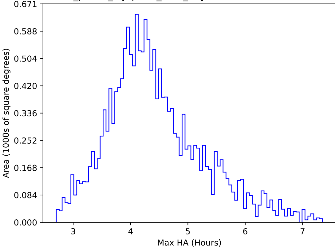
roll_pause_mjdp180_v3.4_10yrs WFD r band: Max HA
