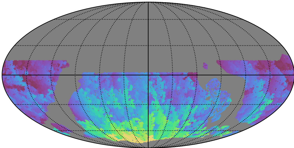
roll_pause_mjdp180_v3.4_10yrs WFD g band: Max HA
