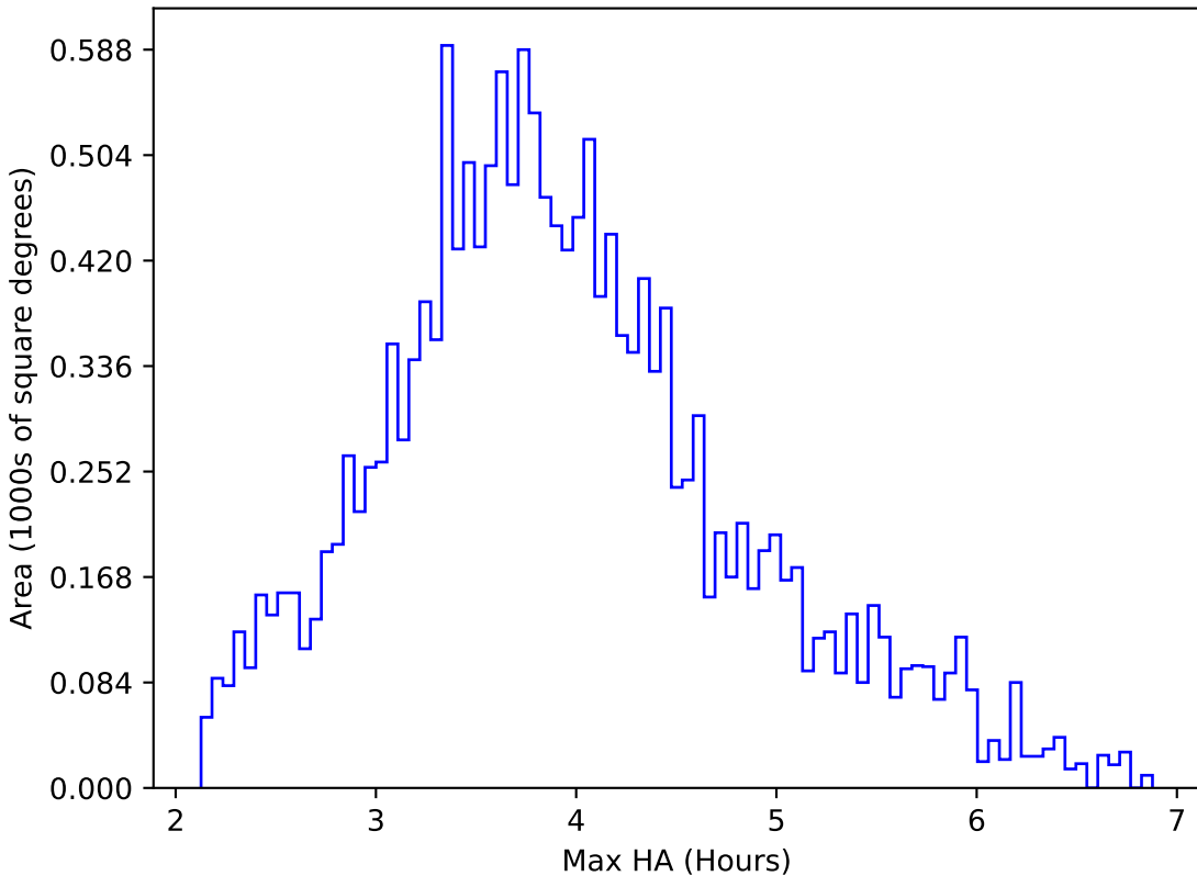
roll_pause_mjdp180_v3.4_10yrs WFD g band: Max HA
