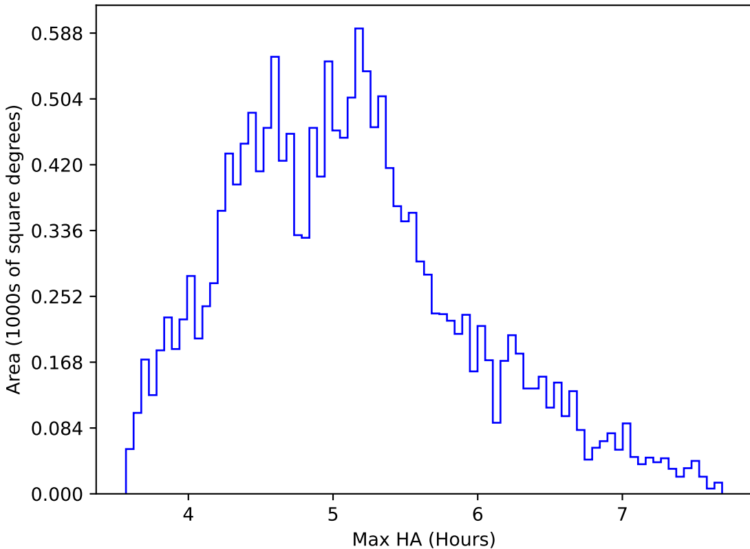
roll_pause_mjdp180_v3.4_10yrs WFD all bands: Max HA
