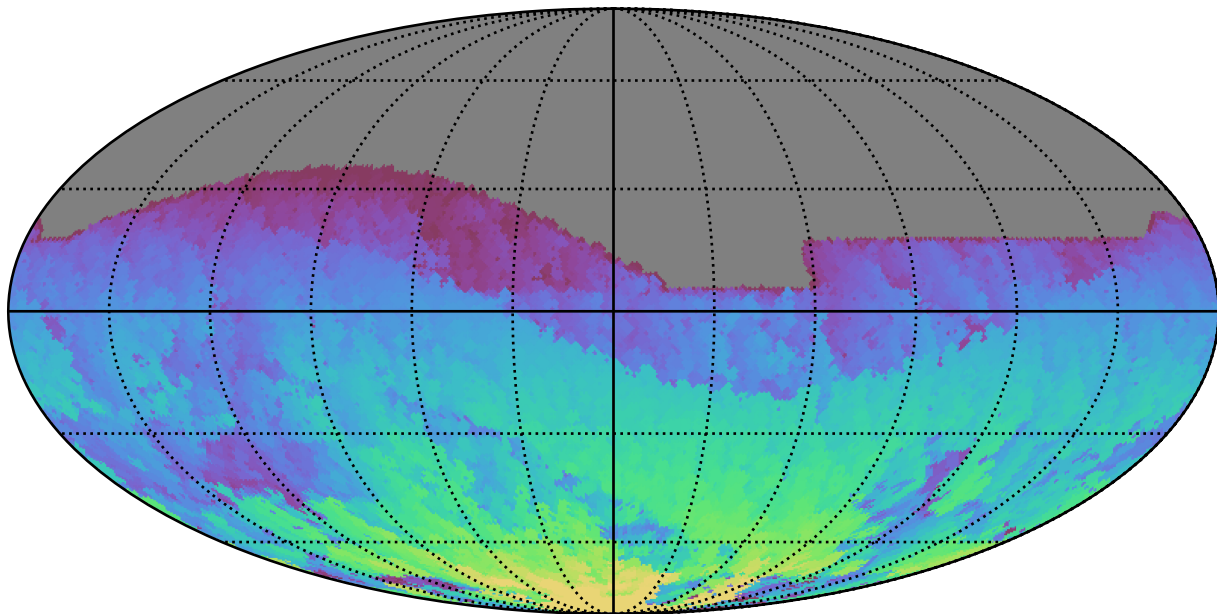
roll_pause_mjdp180_v3.4_10yrs All sky z band: Max HA
