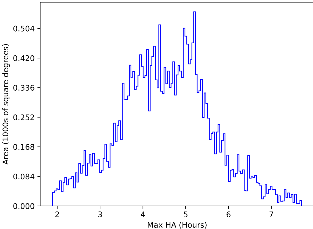
roll_pause_mjdp180_v3.4_10yrs All sky z band: Max HA
