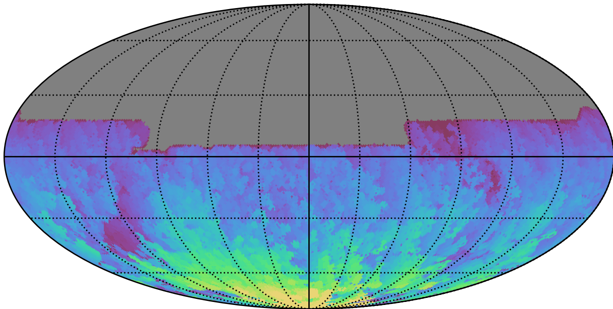
roll_pause_mjdp180_v3.4_10yrs All sky y band: Max HA
