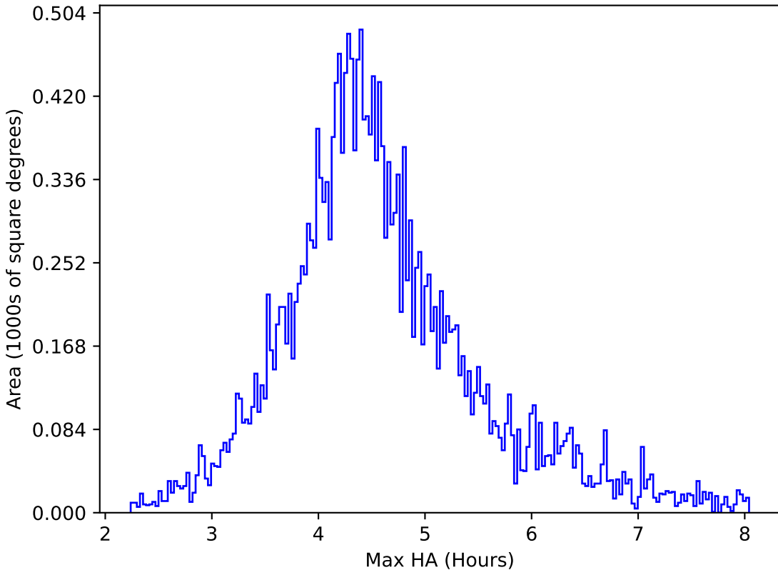
roll_pause_mjdp180_v3.4_10yrs All sky y band: Max HA
