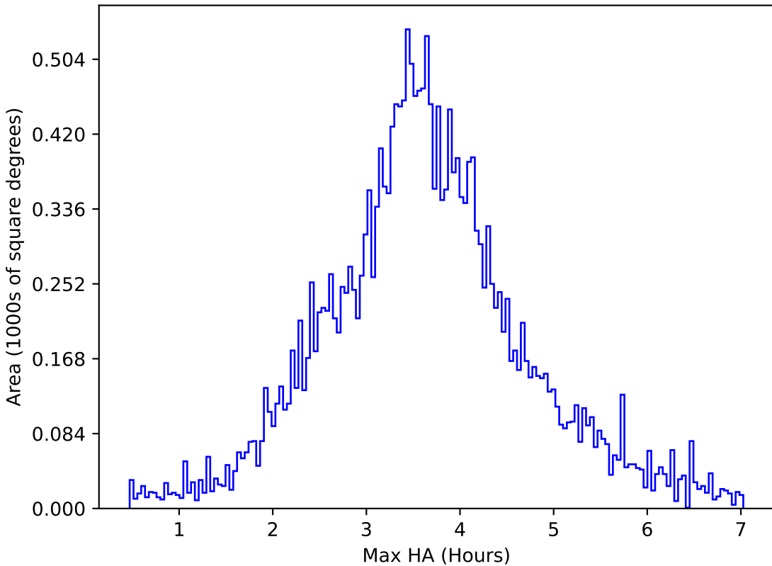
roll_pause_mjdp180_v3.4_10yrs All sky u band: Max HA
