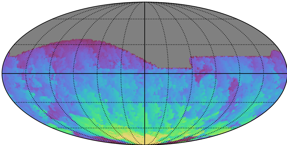
roll_pause_mjdp180_v3.4_10yrs All sky r band: Max HA
