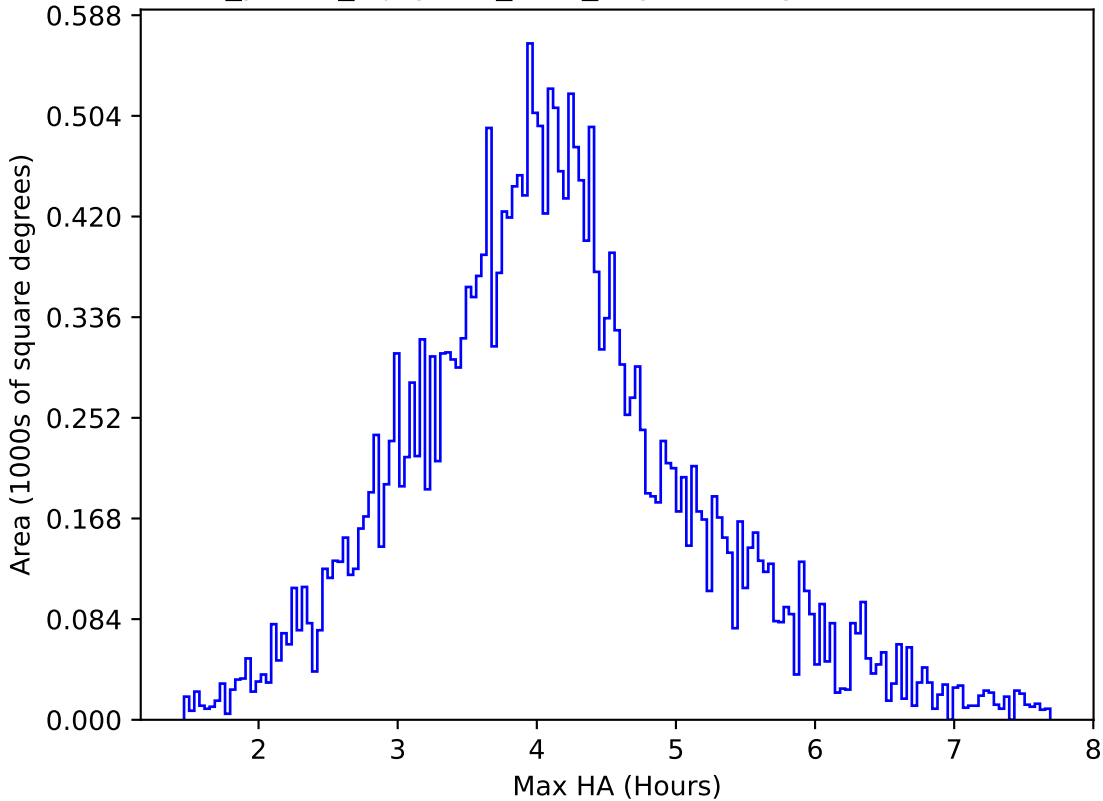
roll_pause_mjdp180_v3.4_10yrs All sky r band: Max HA
