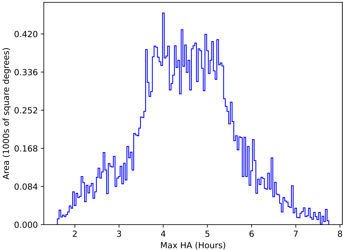
roll_pause_mjdp180_v3.4_10yrs All sky i band: Max HA
