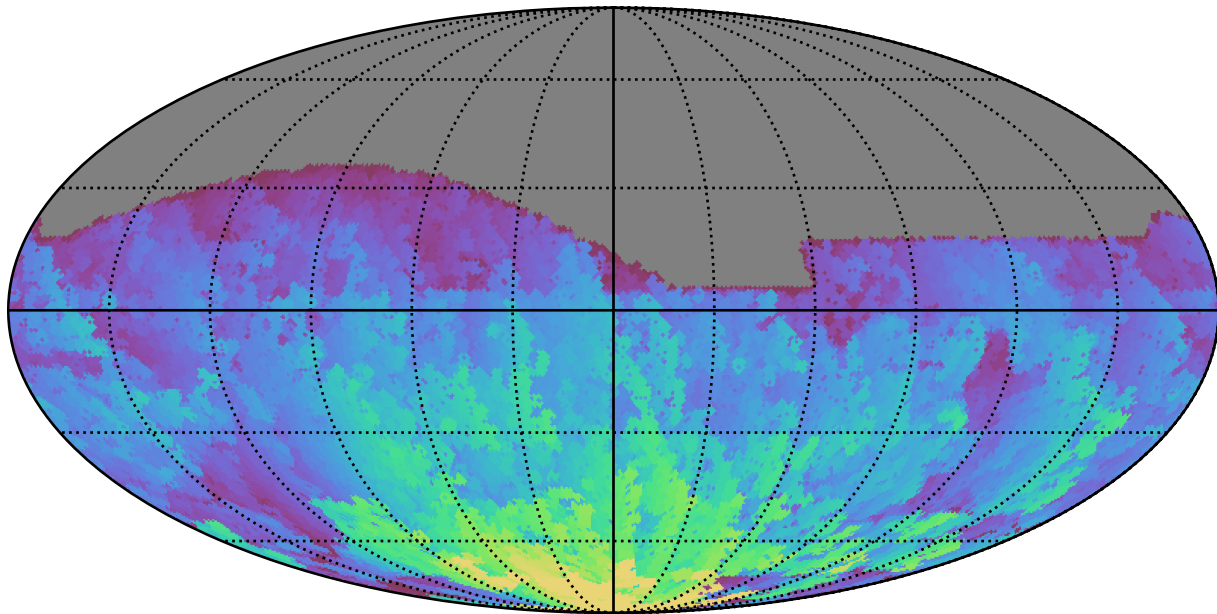
roll_pause_mjdp180_v3.4_10yrs All sky g band: Max HA
