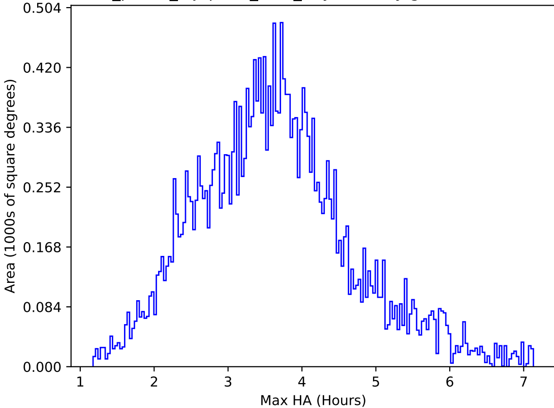
roll_pause_mjdp180_v3.4_10yrs All sky g band: Max HA
