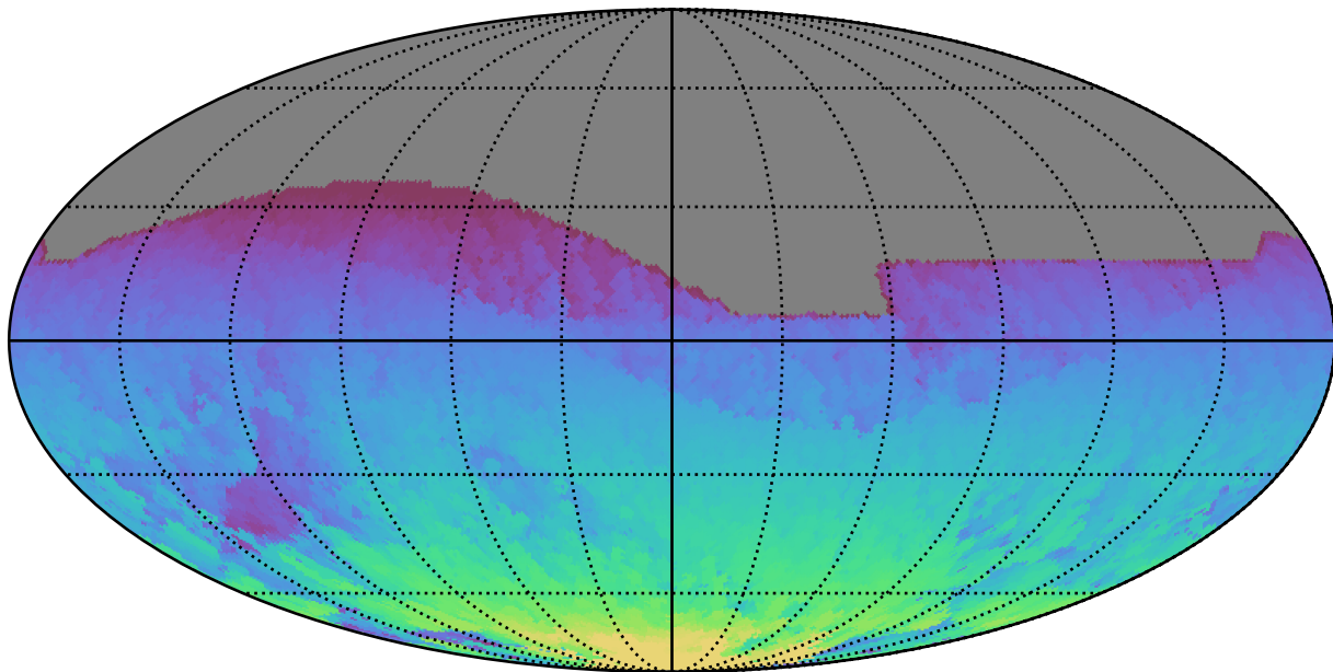
roll_pause_mjdp180_v3.4_10yrs All sky all bands: Max HA
