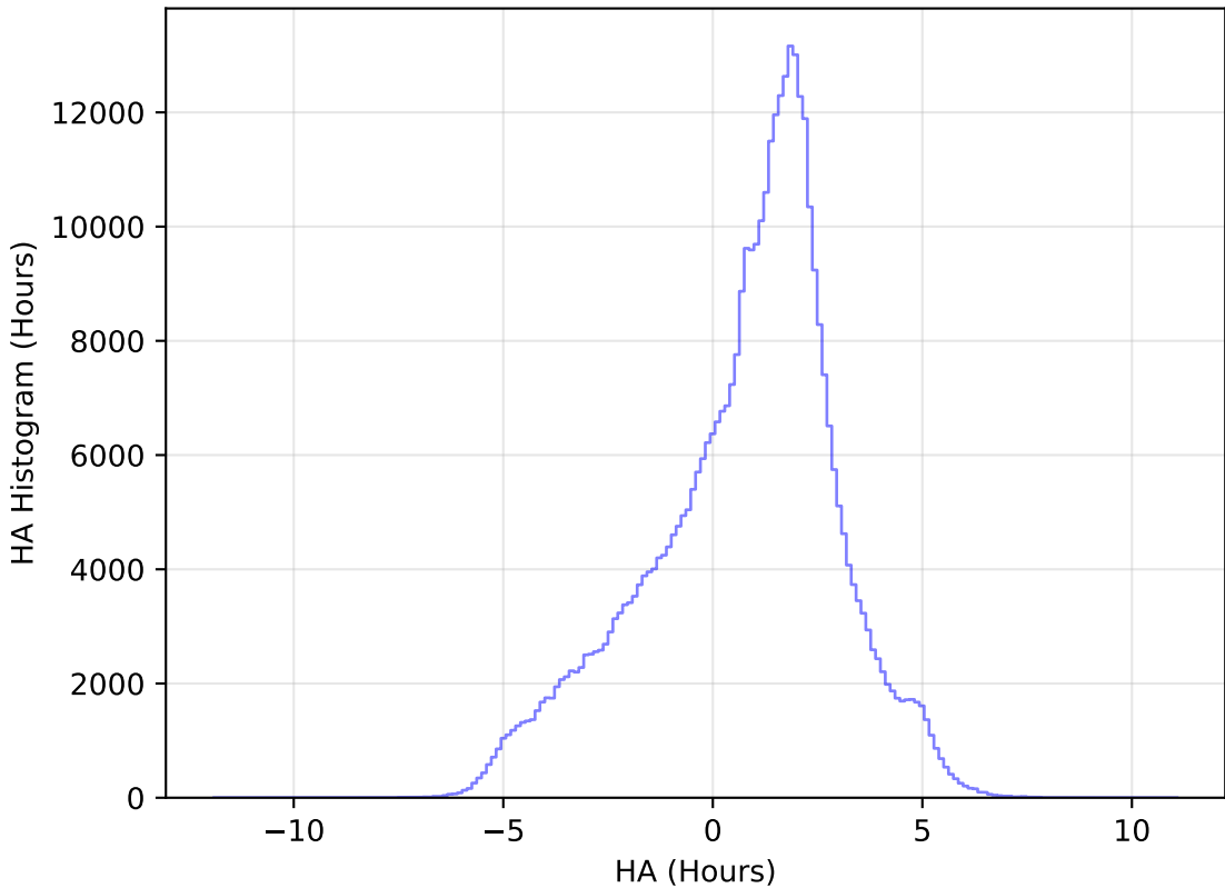
roll_pause_mjdp180_v3.4_10yrs WFD z band: HA Histogram
