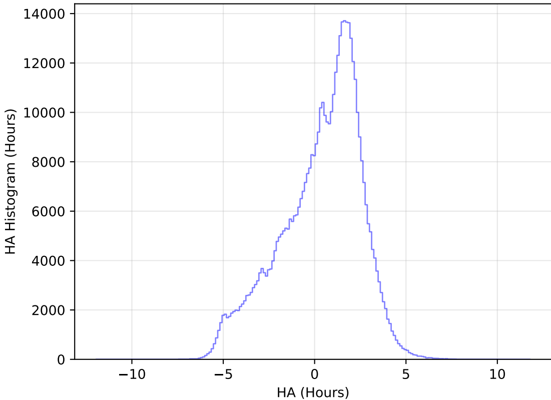
roll_pause_mjdp180_v3.4_10yrs WFD r band: HA Histogram
