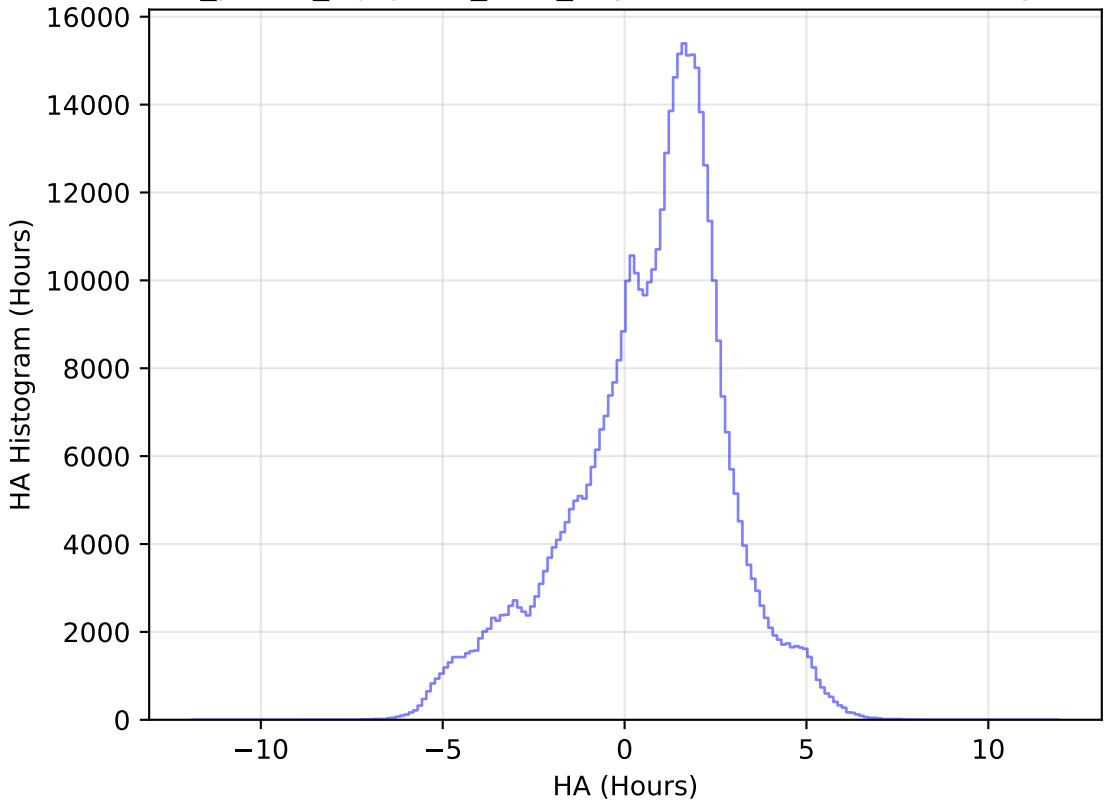
roll_pause_mjdp180_v3.4_10yrs WFD i band: HA Histogram
