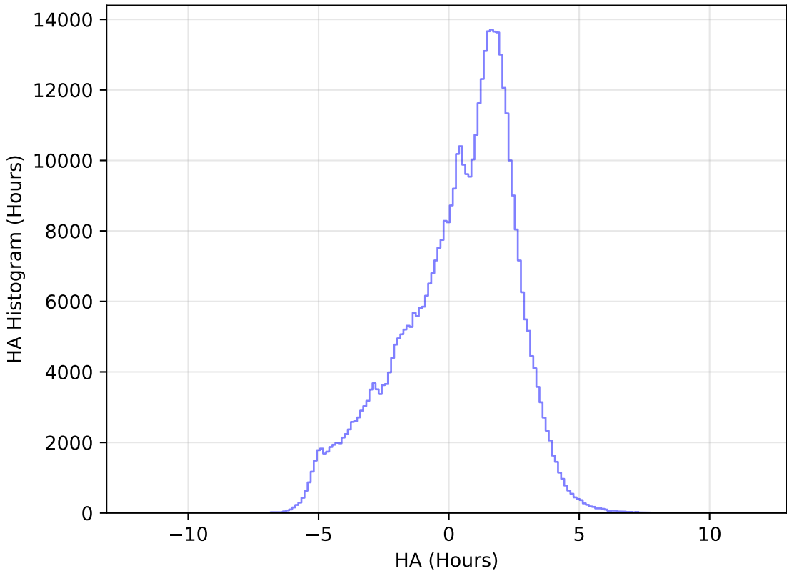
roll_pause_mjdp180_v3.4_10yrs All sky r band: HA Histogram
