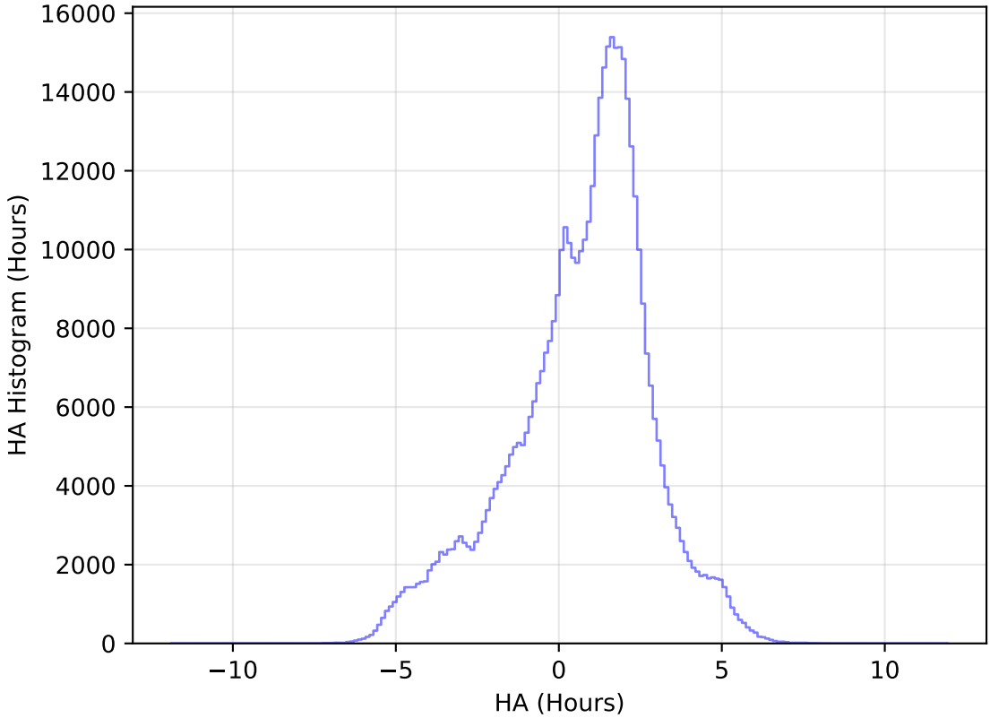
roll_pause_mjdp180_v3.4_10yrs All sky i band: HA Histogram
