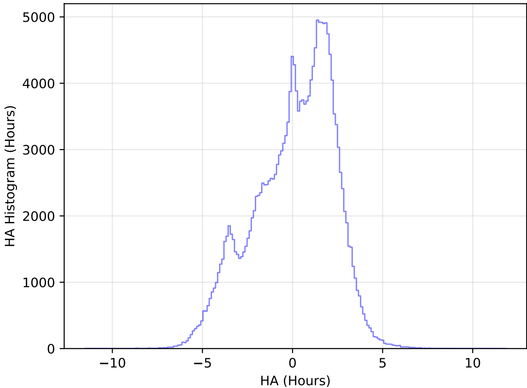
roll_pause_mjdp180_v3.4_10yrs All sky g band: HA Histogram
