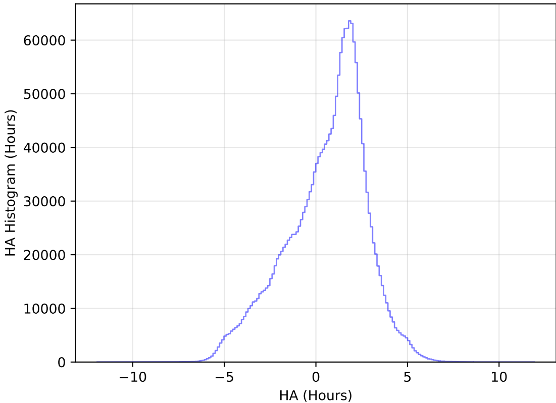
roll_pause_mjdp180_v3.4_10yrs All sky all bands: HA Histogram
