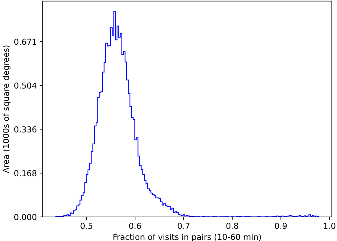
roll_pause_mjdp180_v3.4_10yrs gri WFD: Fraction of visits in pairs (10-60 min)
