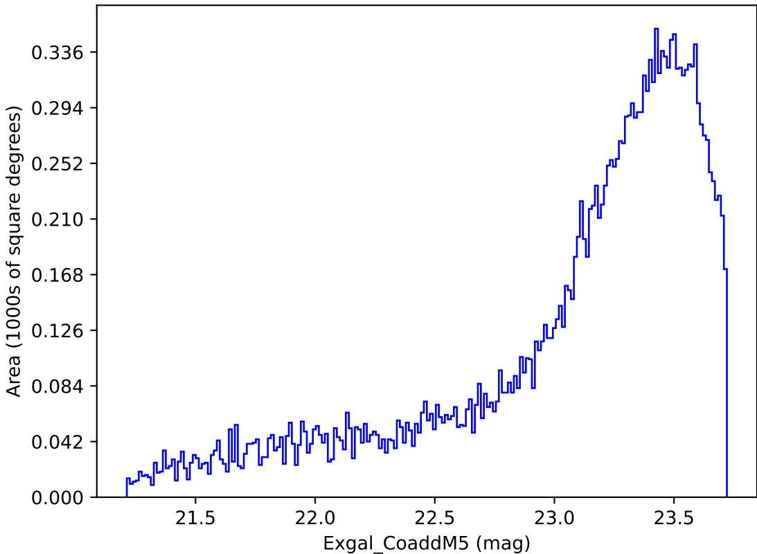
roll_pause_mjdp180_v3.4_10yrs Yr 3-4 y band: Exgal_CoaddM5
