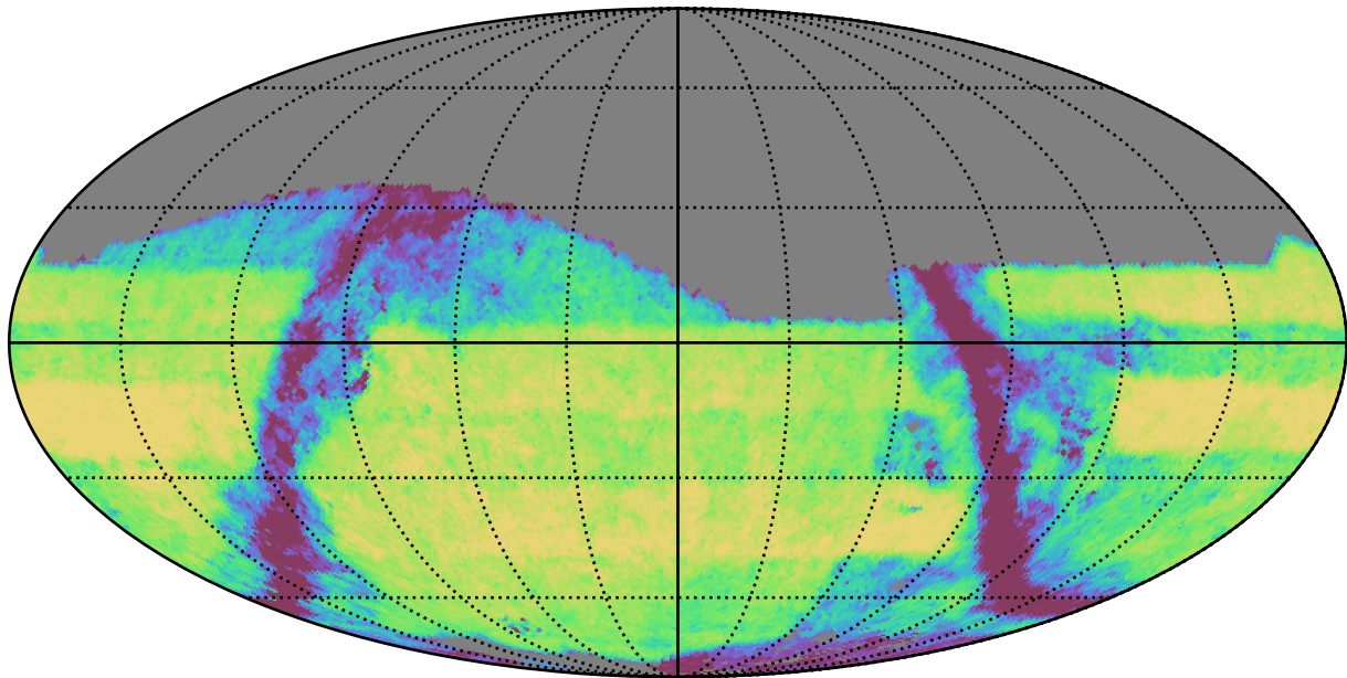
roll_pause_mjdp180_v3.4_10yrs Yr 3-4 i band: Exgal_CoaddM5
