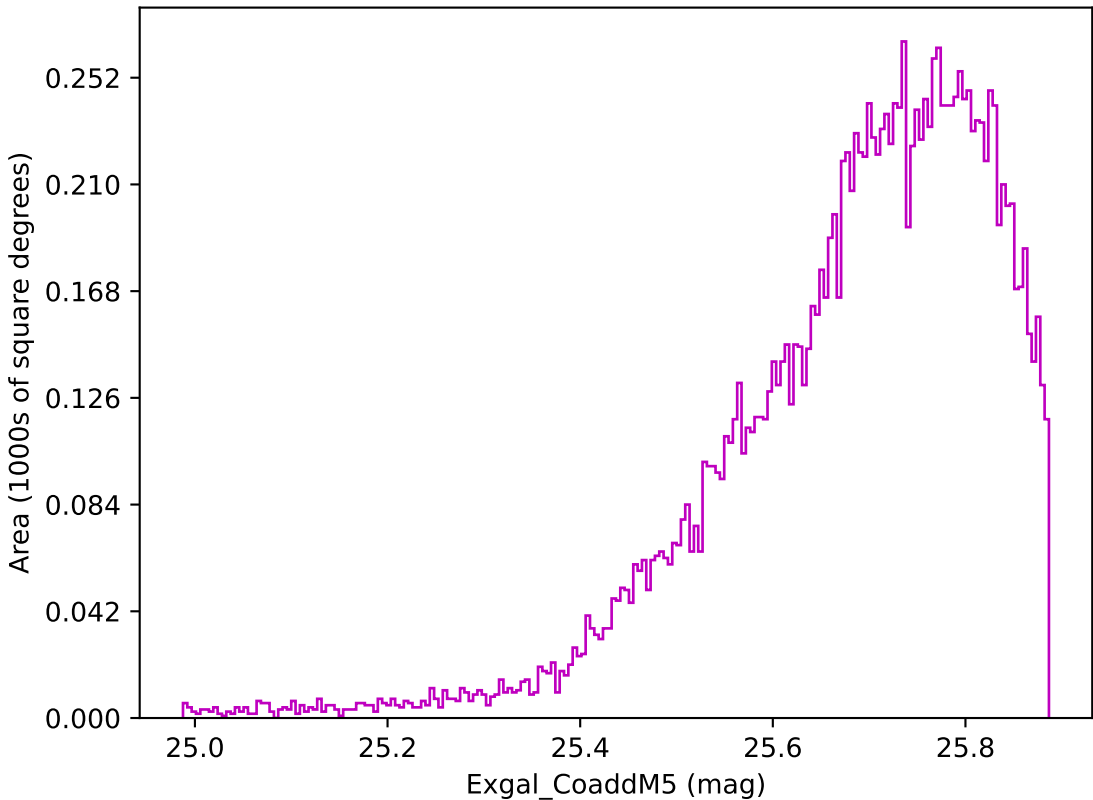
roll_pause_mjdp180_v3.4_10yrs WFD z band: Exgal_CoaddM5
