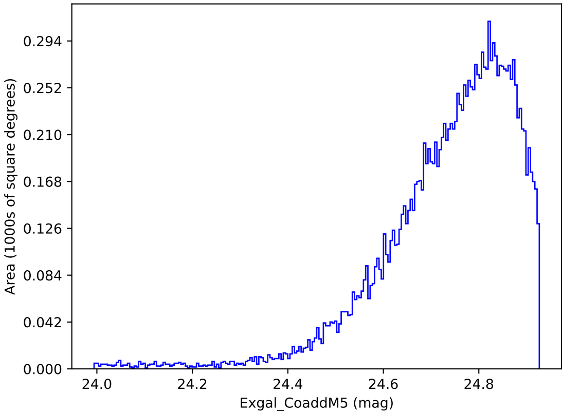
roll_pause_mjdp180_v3.4_10yrs WFD y band: Exgal_CoaddM5
