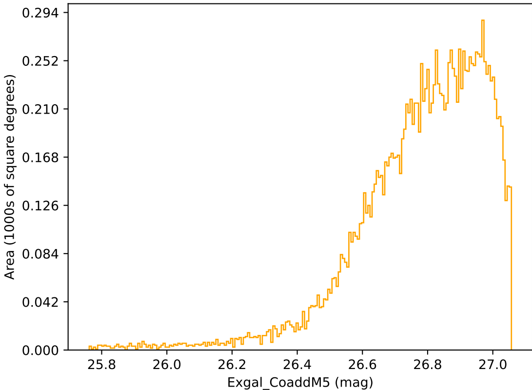
roll_pause_mjdp180_v3.4_10yrs WFD r band: Exgal_CoaddM5
