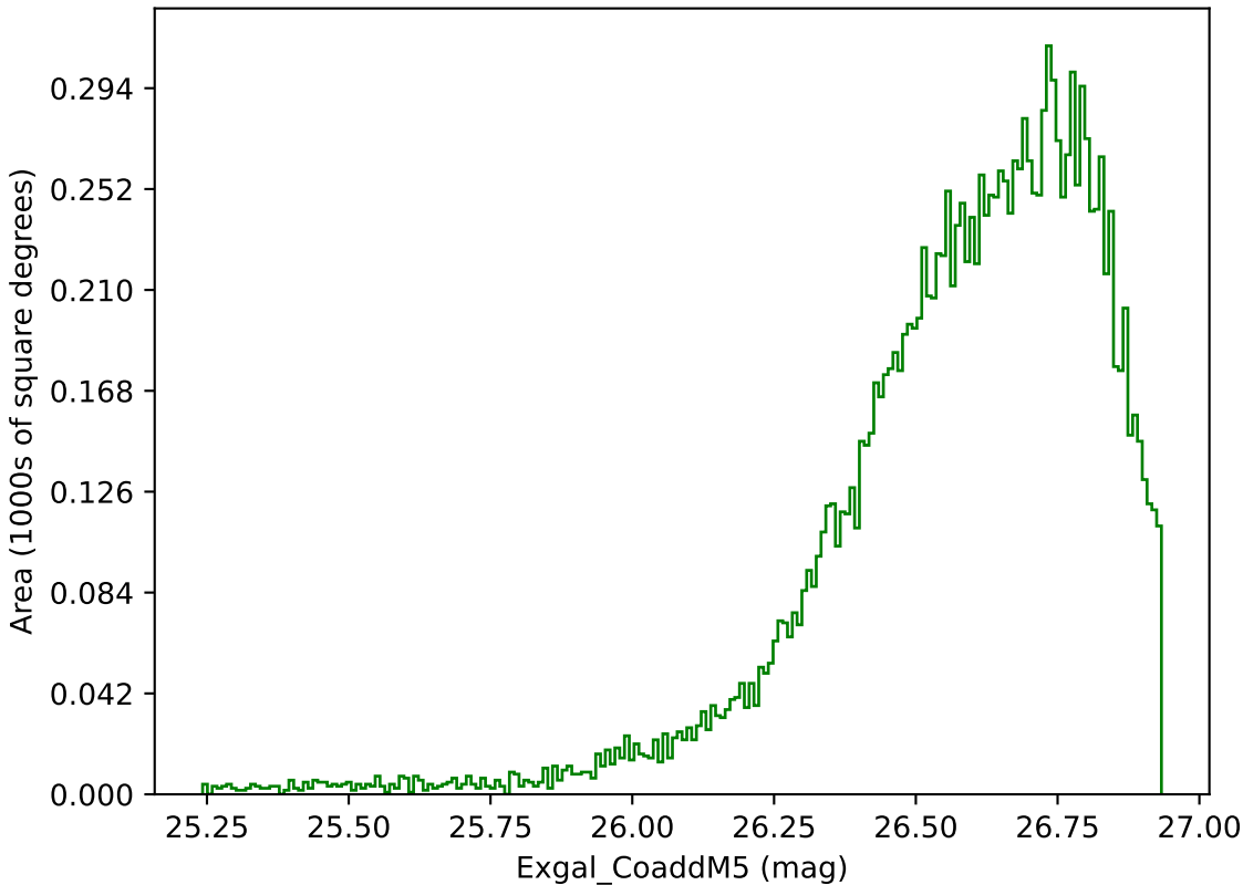
roll_pause_mjdp180_v3.4_10yrs WFD g band: Exgal_CoaddM5
