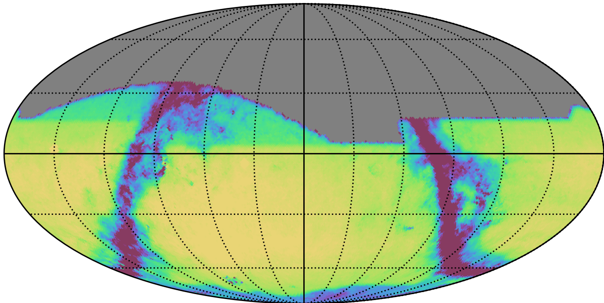
roll_pause_mjdp180_v3.4_10yrs All sky r band: Exgal_CoaddM5
